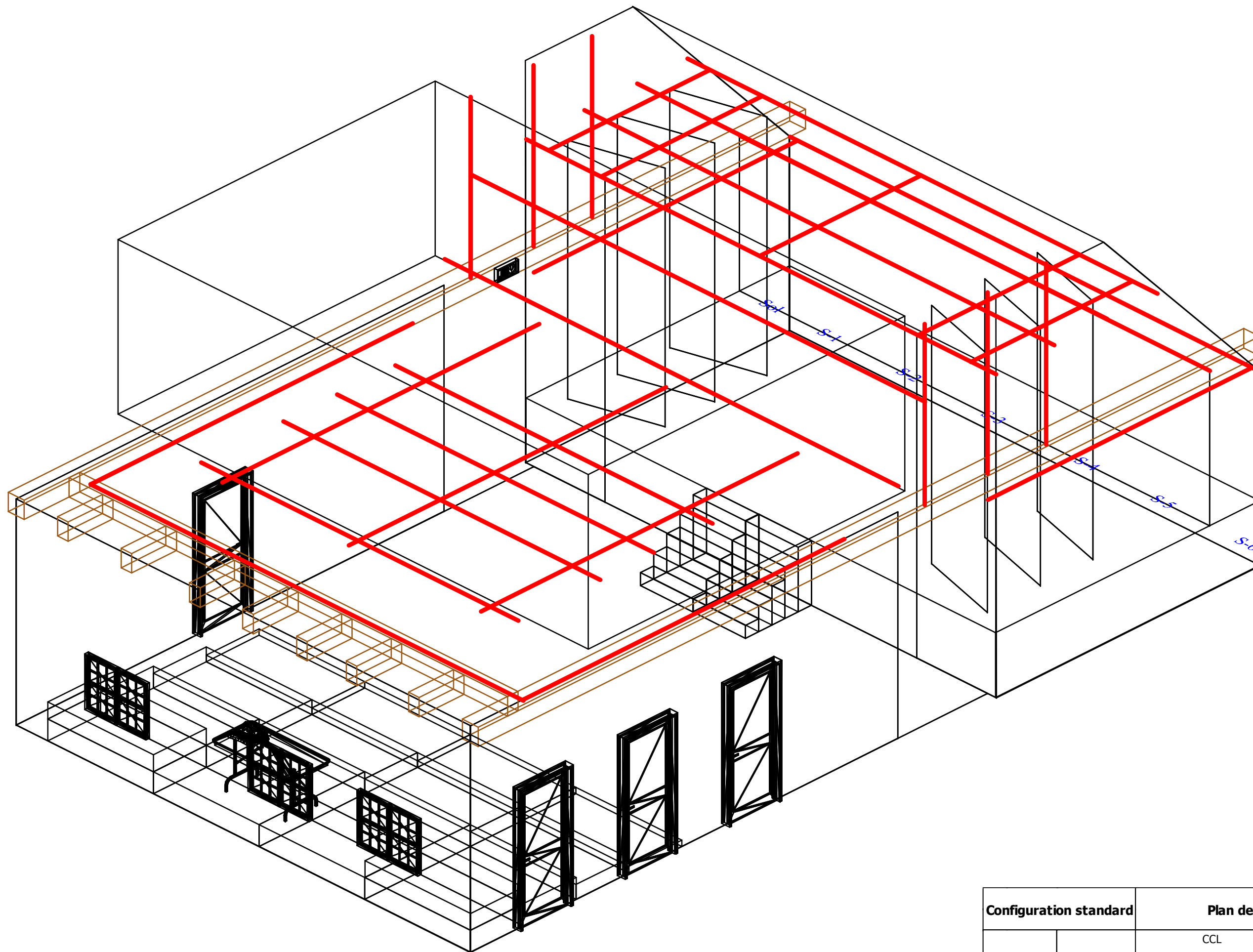
Plan - Isometric
